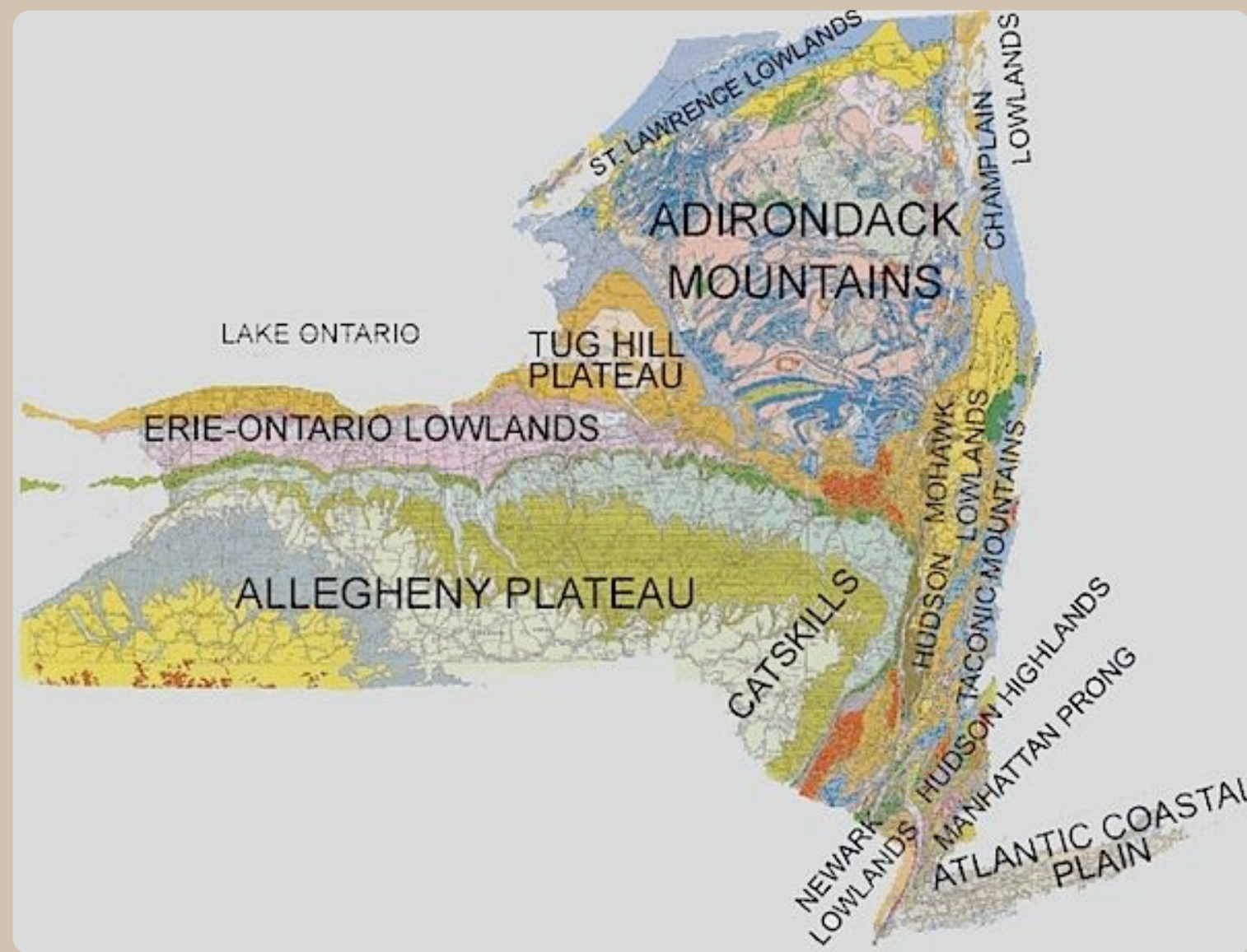
The Tug Hill Plateau is centrally located within NY State.
